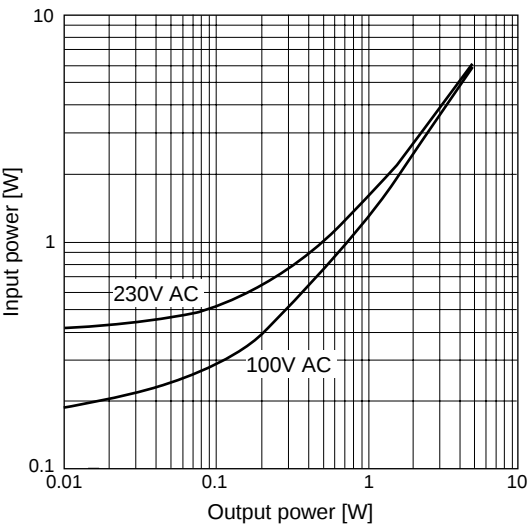
Input power vs. output power
