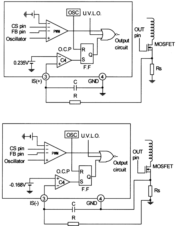
Fig. 14 Overcurrent limiting circuit
