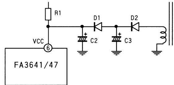
Fig. 23 Startup circuit (3)
