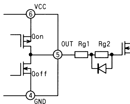
Fig. 36 Gate circuit
