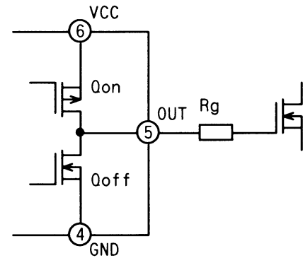
Fig. 35 Output stage
