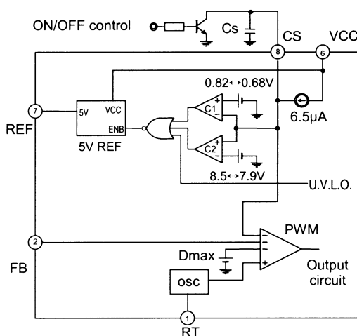
Fig. 12 External output ON/OFF control circuit
