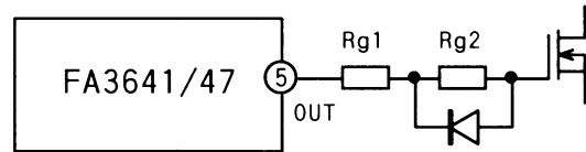
Fig. 34 Gate circuit
